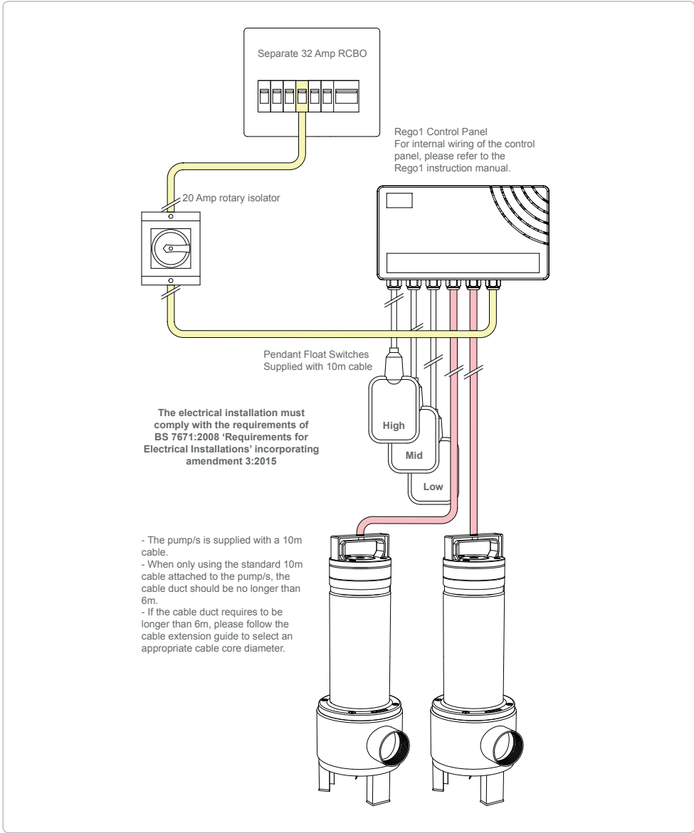
Figure 1. Rego1 typical wiring schematic
