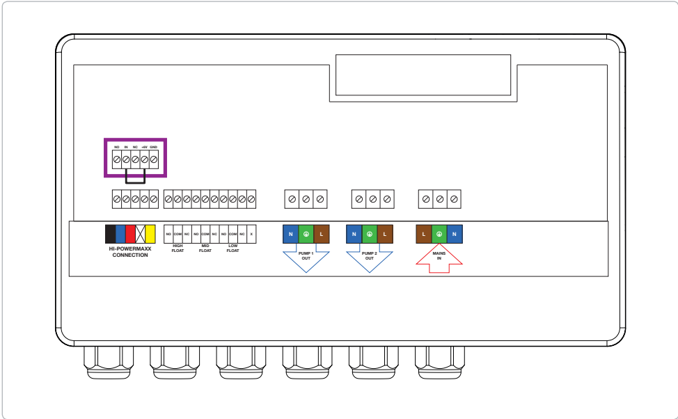
Figure 5. Typical Volt Free Relay (VFR) connection link
