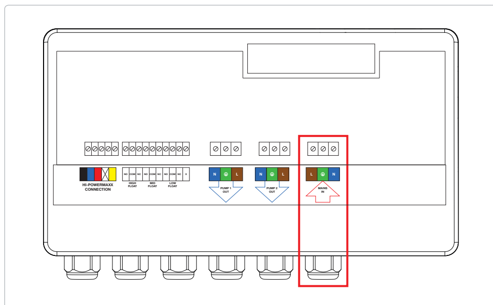
Figure 2. Connecting mains power
